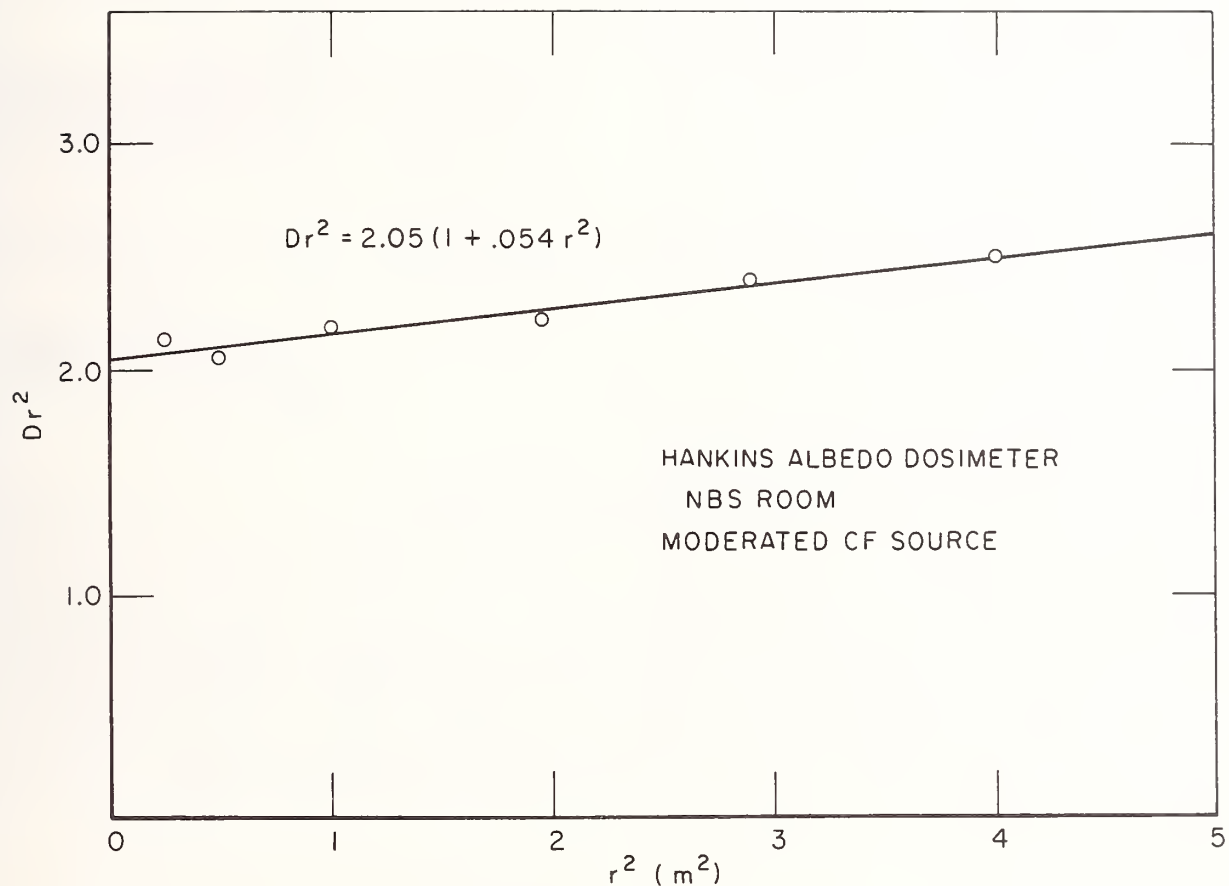
Figure 3 - Response of the Hankins Albedo Dosimeter per unit dose equivalent as a function of distance from the neutron source. The measurements were taken with a moderated ^{252}\text{Cf} source in the NBS calibration room. The data are fitted to an equation of the form
